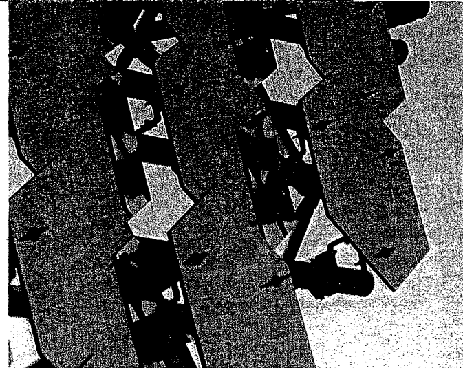
Physicists prepare one of the Auger Observatory's tanks. Below: The mirrors of VERITAS telescopes have helped scientists detect cosmic-ray emitters. Opposite: A map of the southern sky shows the correlation between sources of incoming cosmic rays (circles) and the locations of active galaxies (red dots).
